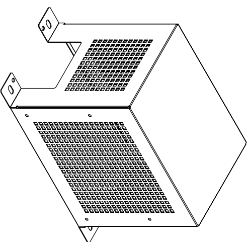
isometric M1:5
