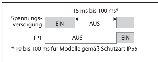
Abb. 5-293: IPF-Signal
