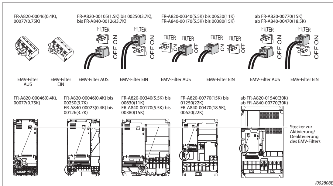
Abb. 3-7: Internes EMV-Filter
